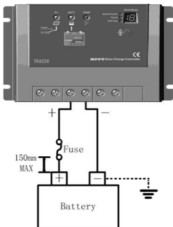
Figure 3-2 Battery wiring
